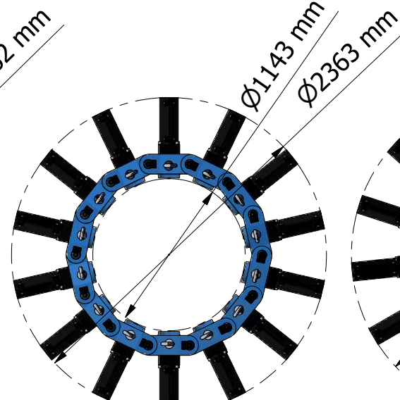
14 Link Assy 1540kg
