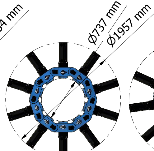
10 Link Assy 1100kg
