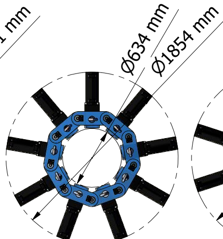
9 Link Assy 990kg
