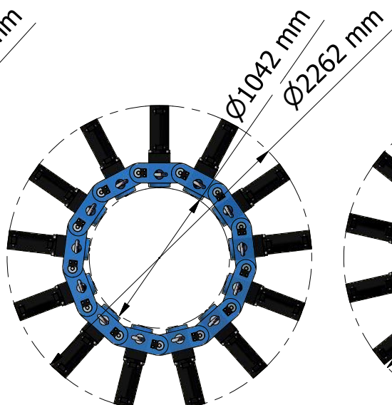
13 Link Assy 1430kg
